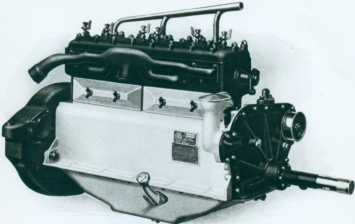
Left side view of the Red Seal Continental Seven-R Motor
