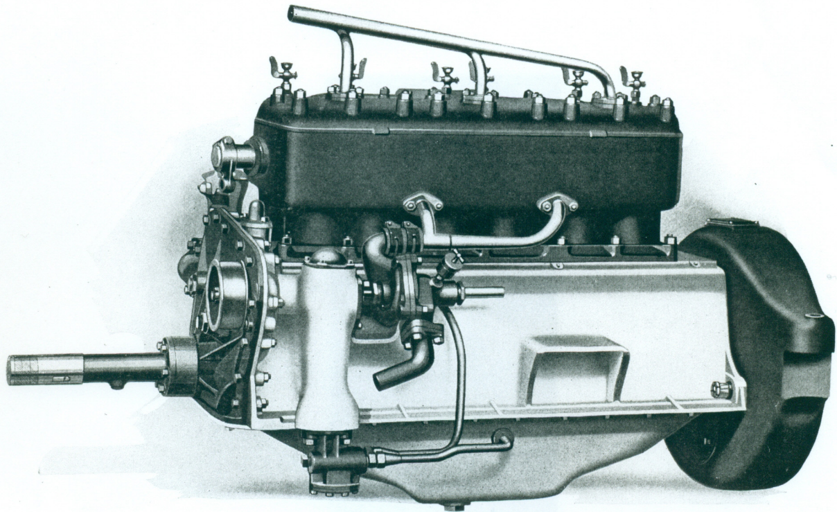
Right side view of the Red Seal Continental Seven-R Motor
